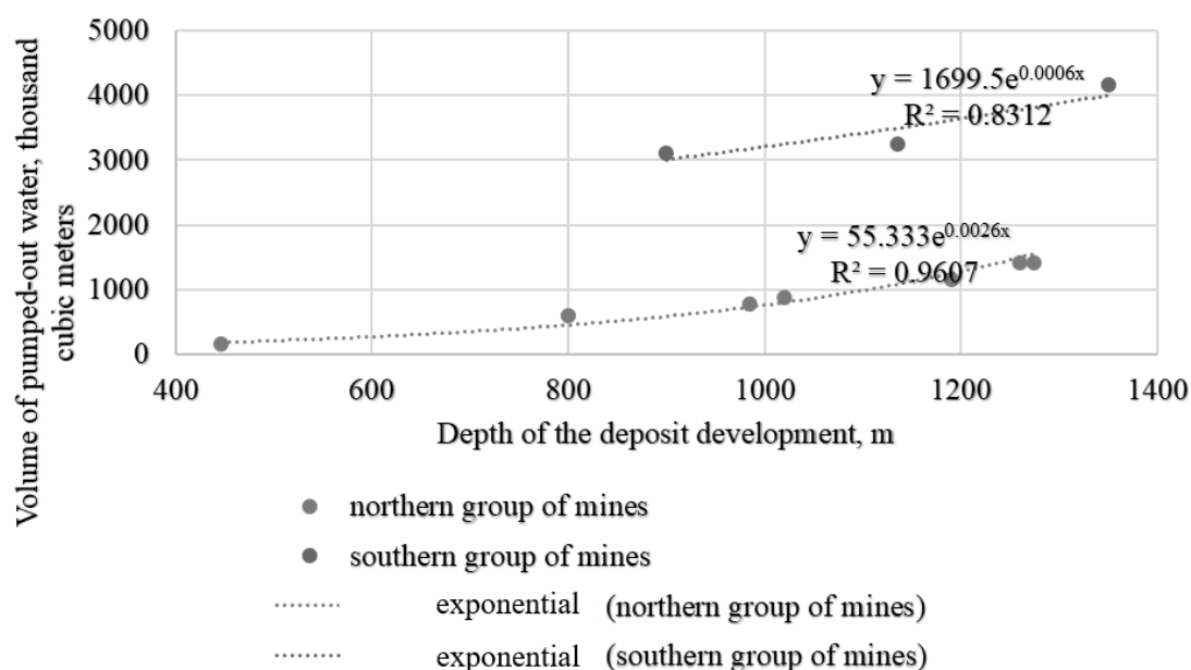
Figure 4 – Dependence of water inflows on the depth of the deposit development
